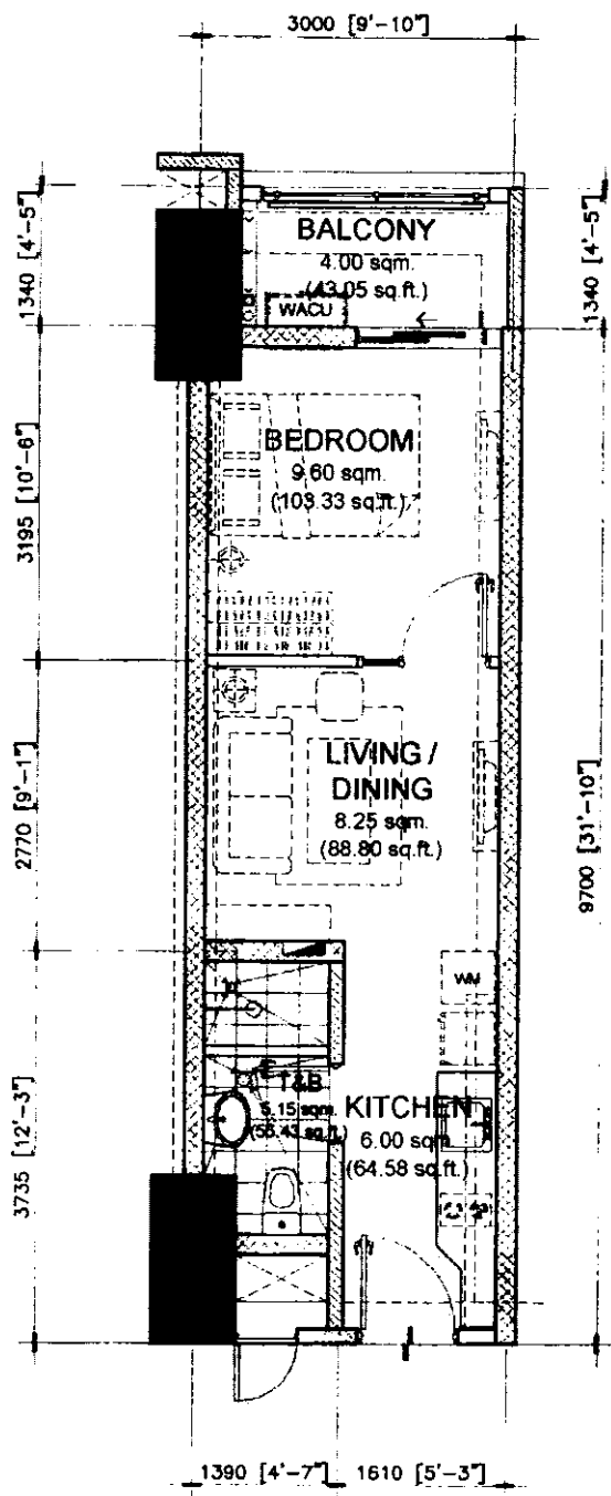
29.00 sq.m. 1-BR TYPE - B.1 INNER UNIT - 29.00 sq.m. / 312.15 sq.ft. WITH BALCONY - 4.00 sq.m/ 43.05 sq.ft. GROSS FLOOR AREA - 33.00 sq.m. / 355.20 sq.ft
