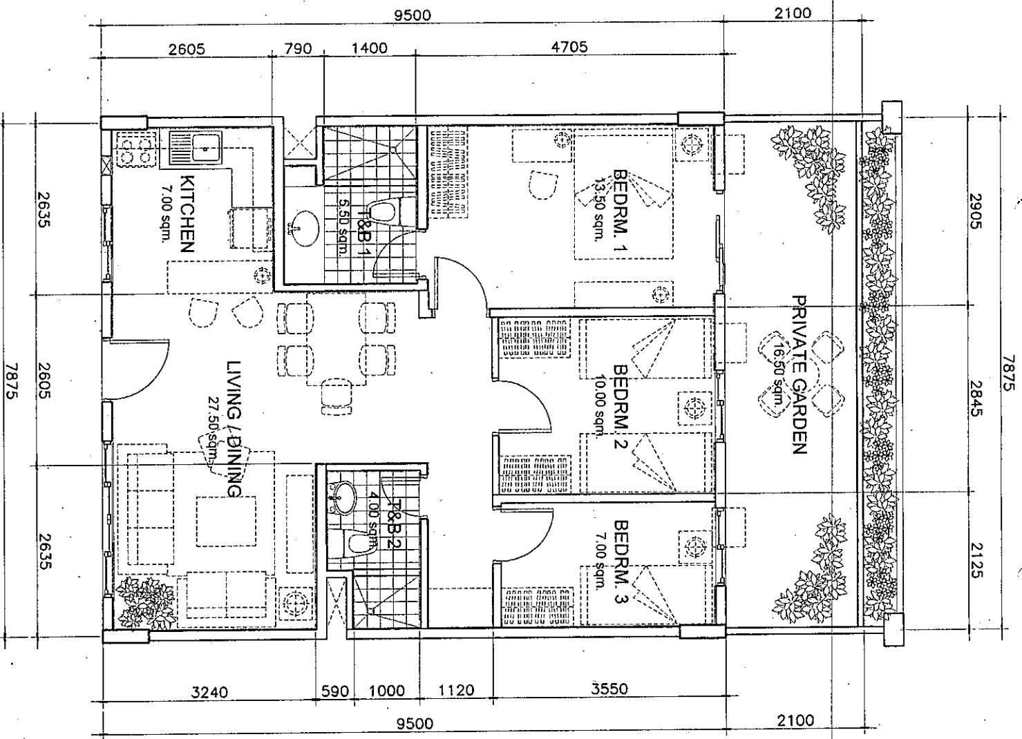
MID UNIT (74.50 sq.m.) WITH PRIVATE GARDEN (A = 16.50 sq.m.) SCALE: 1:80 mtrs.
