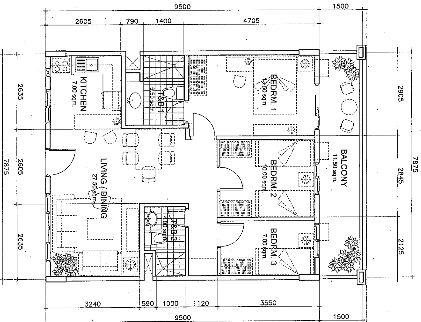
MID UNIT (74.50 sq.m.) WITH BALCONY (A = 11.50sq.m.)
