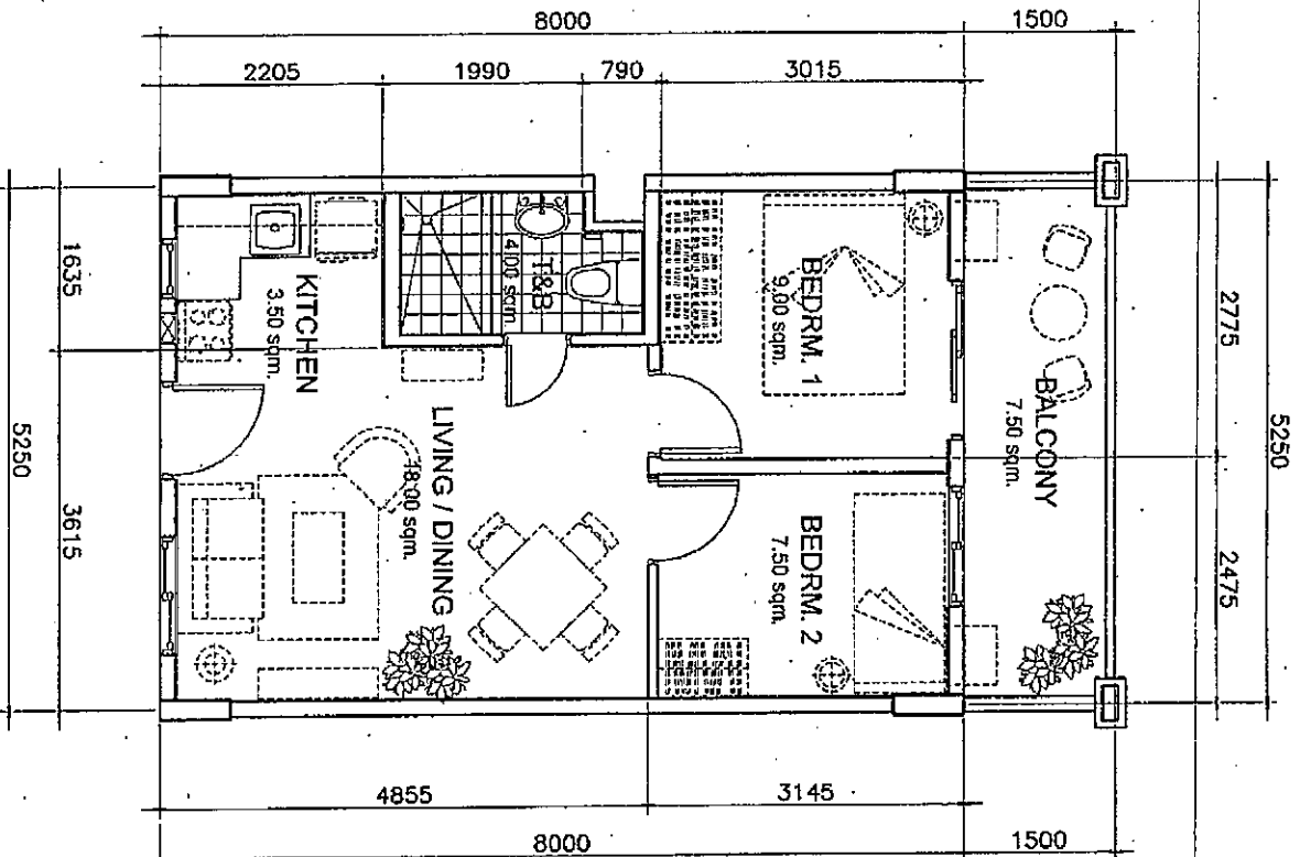
MID UNIT (42.00 sq.m.) WITH BALCONY (A = 7.50 sq.m.)
